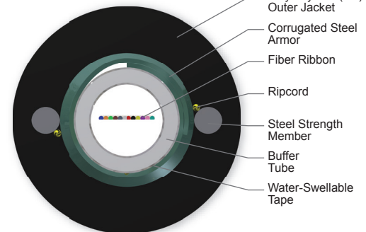
Cross Section of Part Number: 012EC5-14100D53
