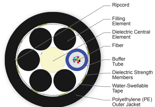
Cross Section of Part Number: 012EN4-T4S01A20
