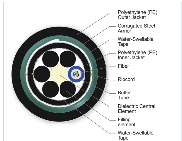
Cross Section of Part Number: 012EU5-T4101C20
