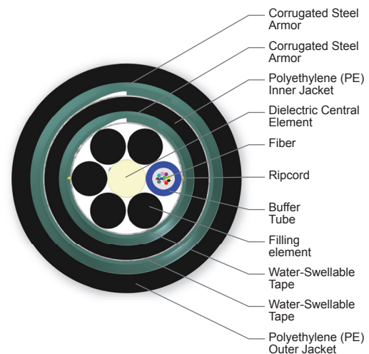
Cross Section of Part Number: 012EUD-T4101A20
