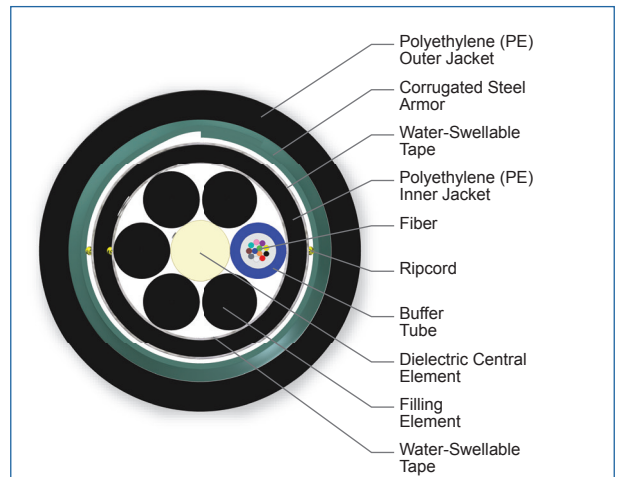
Cross Section of Part Number: 012KU5-T4130C20
