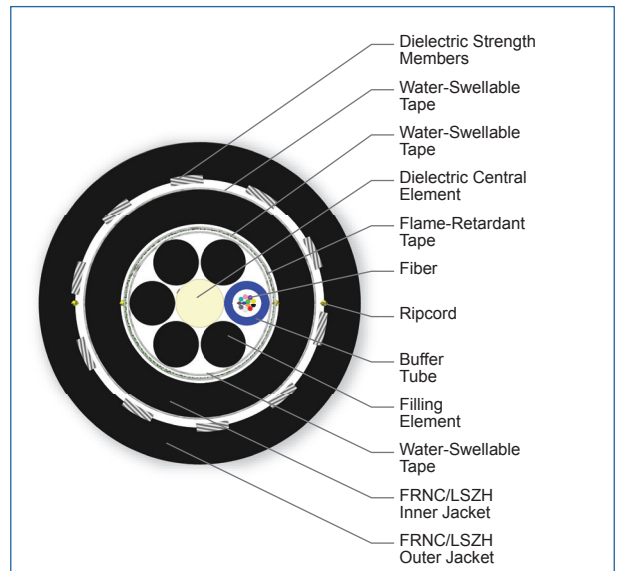
Cross Section of Part Number: 012KUL-T3630D2M
