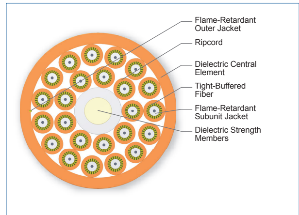
Cross Section of Part Number: 024K61-31330-24
