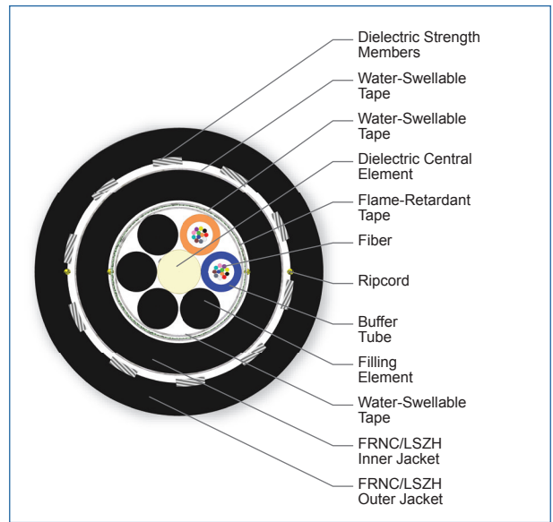
Cross Section of Part Number: 024KUL-T3630D2M
