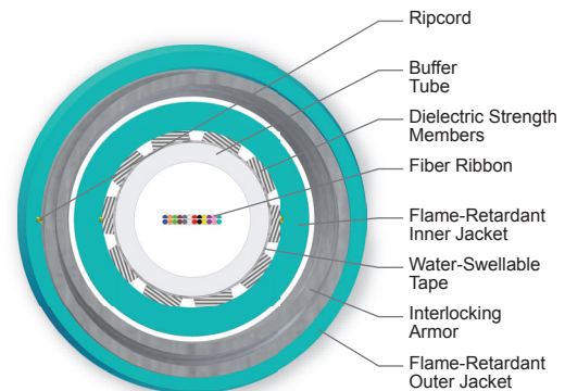
Cross Section of Part Number: 024TC8-14190-A3
