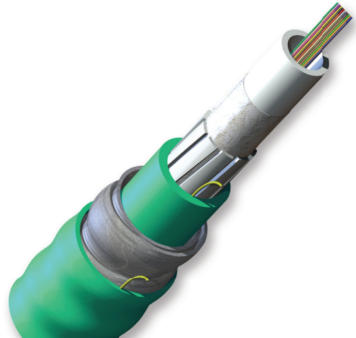
Part Number: 024TC8-14190-A3
