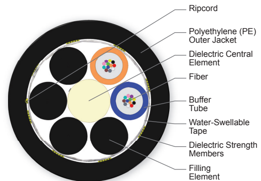
Cross Section of Part Number: 024TN4-T4S31A20
