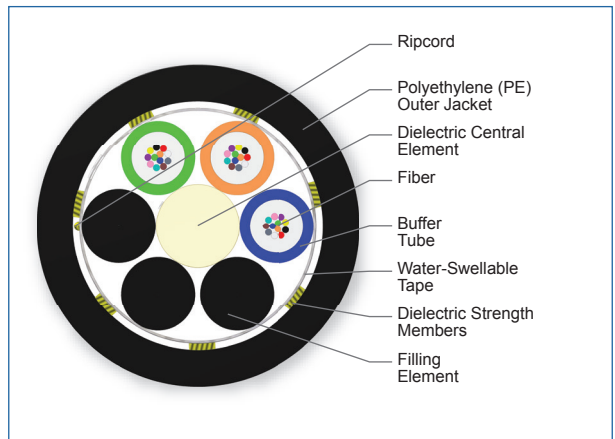
Cross Section of Part Number: 036TN4-T4M90A20
