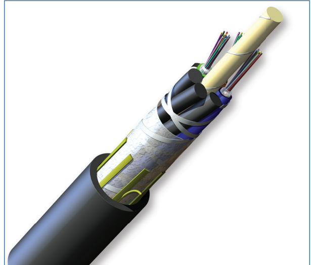
Part Number: 036TN4-T4M90A20
