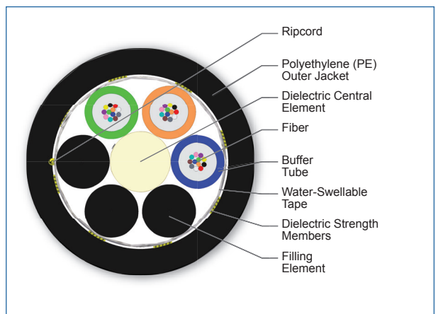
Cross Section of Part Number: 036TN4-T4S31A20
