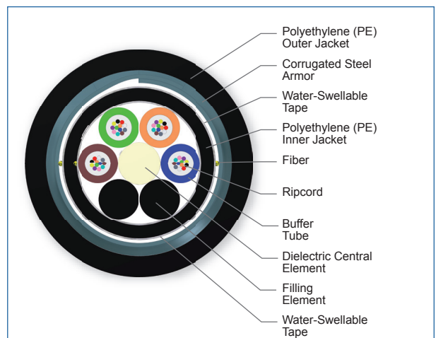
Cross Section of Part Number: 048EU5-T4101C20
