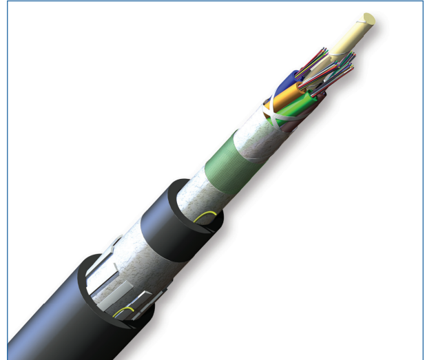
Part Number: 048KUL-T3630D2M
