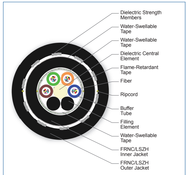
Cross Section of Part Number: 048KUL-T3630D2M
