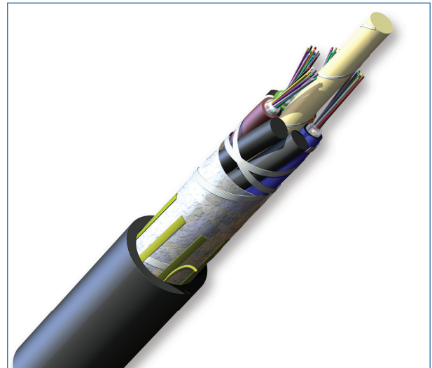
Part Number: 048TN4-T4S90A20
