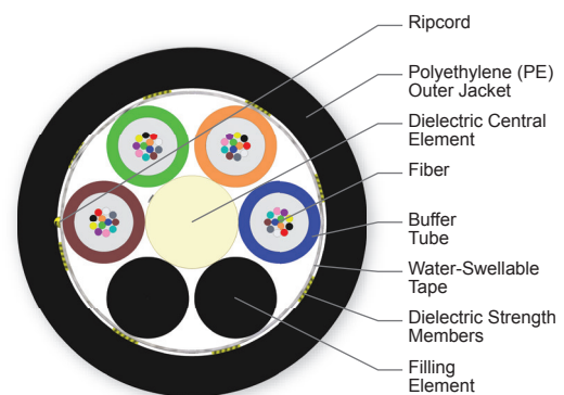
Cross Section of Part Number: 048TN4-T4S90A20
