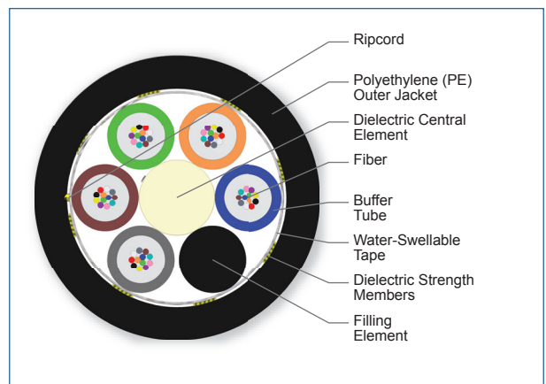
Cross Section of Part Number: 060KN4-T4S30A20
