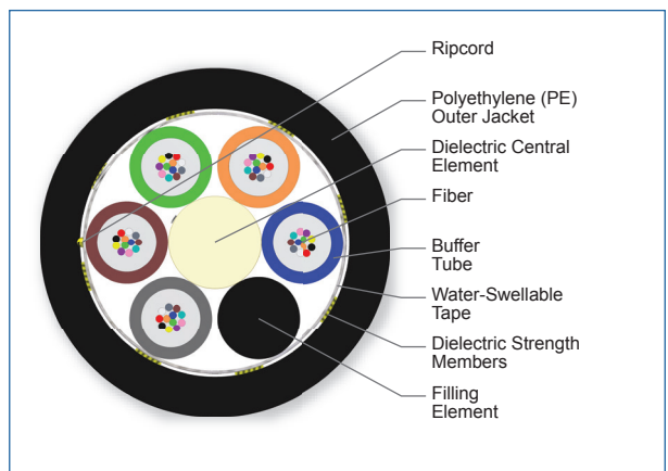
Cross Section of Part Number: 060TN4-T4S90A20
