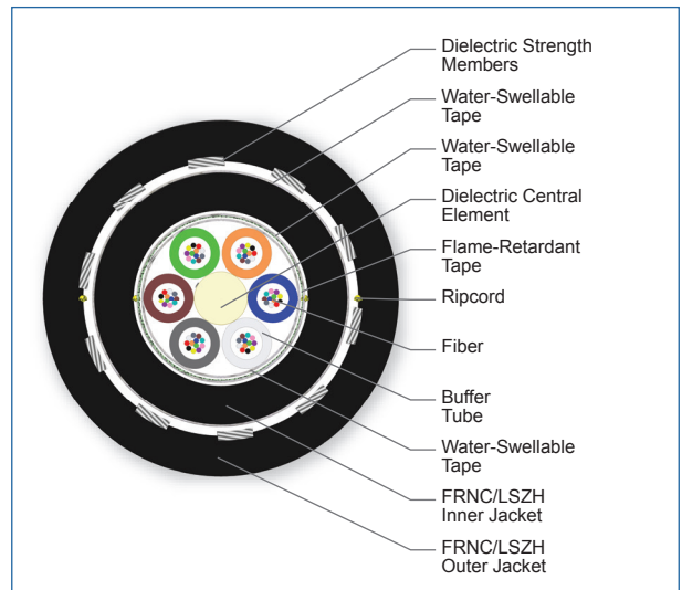
Cross Section of Part Number: 072KUL-T3630D2M
