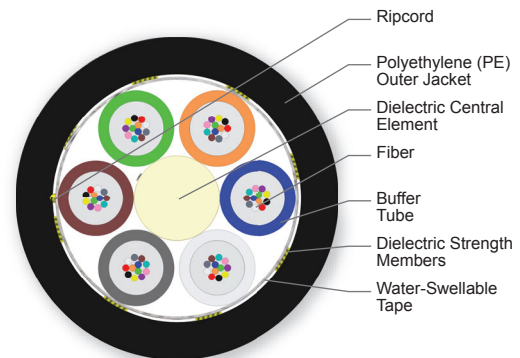
Cross Section of Part Number: 072TN4-T4S90A20
