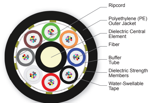
Cross Section of Part Number: 096EN4-T4M01A20
