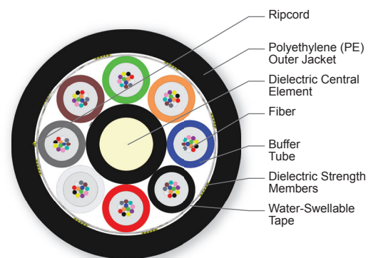
Cross Section of Part Number: 096TN4-T4S31A20
