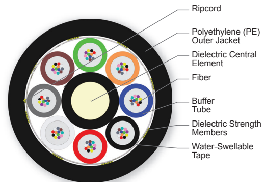
Cross Section of Part Number: 096TN4-T4S80A20
