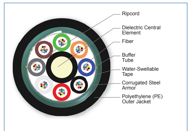
Cross Section of Part Number: 096TUC-T4131D20
