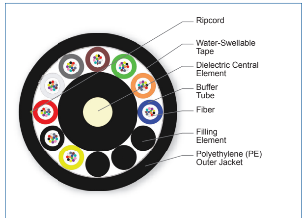
Cross Section of Part Number: 108TU4-T4180D20
