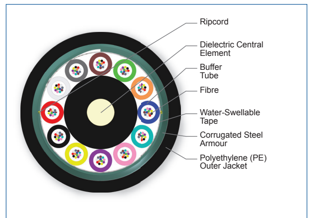
Cross Section of Order Number: 144EUC-T4101F20
