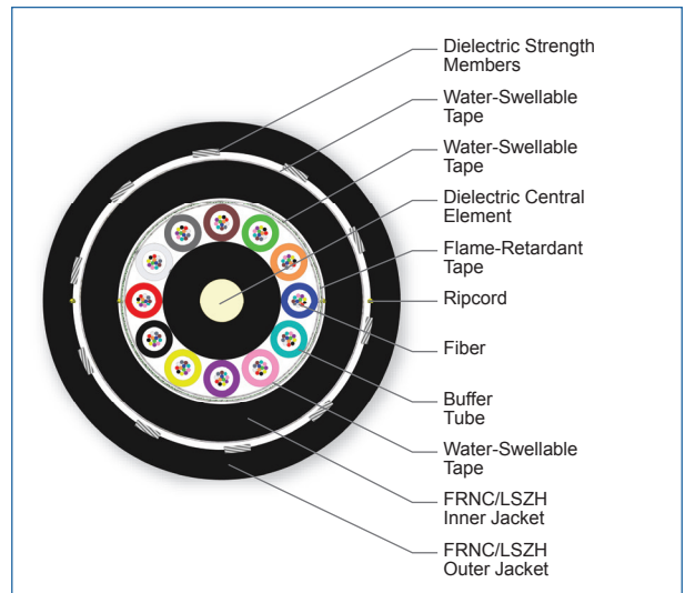
Cross Section of Part Number: 144KUL-T3630D2M
