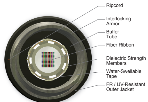
Cross Section of Part Number: 144TCF-14190-A1
