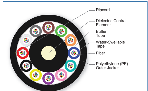
Cross Section of Part Number: 144TU4-T4191D20
