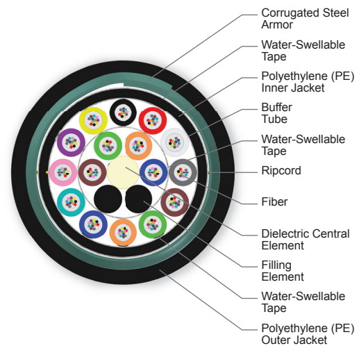
Cross Section of Part Number: 192EU5-T4101C20
