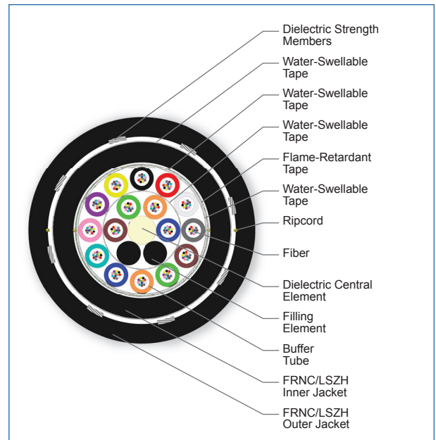
Cross Section of Part Number: 192KUL-T3630D2M
