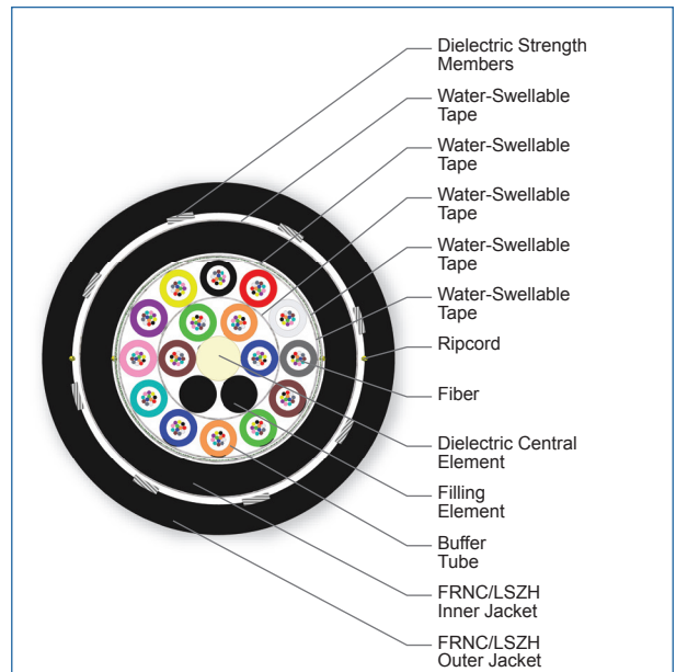
Cross Section of Part Number: 192KUL-T4630D2N
