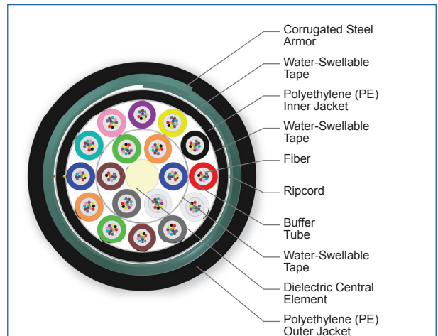
Cross Section of Part Number: 216EU5-T4101C20
