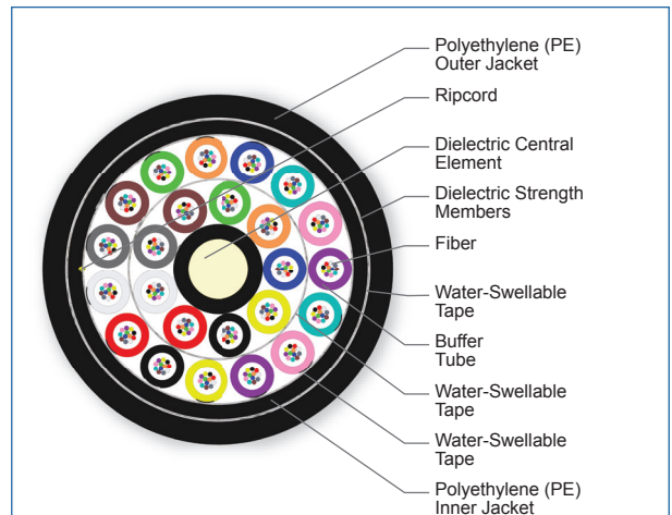
Cross Section of Part Number: 288EUE-T4101D20
