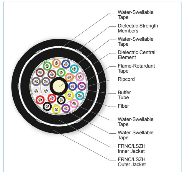
Cross Section of Part Number: 288TUL-T3631D2M
