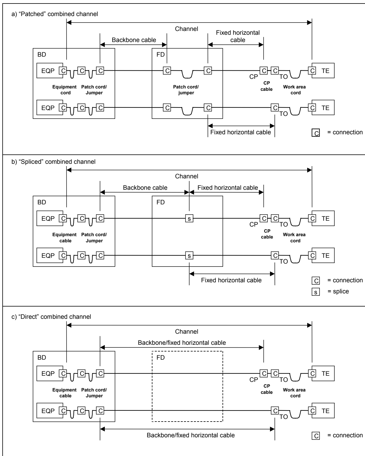
Figure 14 – Combined backbone/horizontal channels
